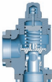
BV2 cutaway
